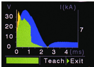
Weld Monitor
